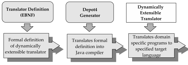
Figure 3. Translator Generation
