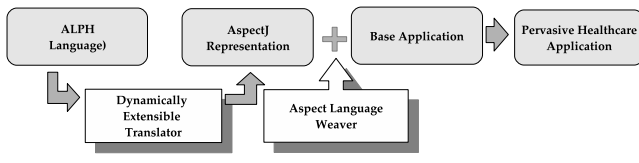
Figure 2. DSL Translation
